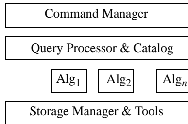
Figure 2: Rough architecture of the kernel
